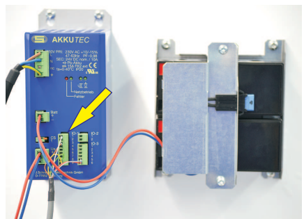
Connect the RS232 interface cable. (Art. No. PSDP0324G100X)
