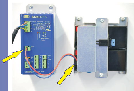
Connect the battery to the battery connector of the AKKUTEK
