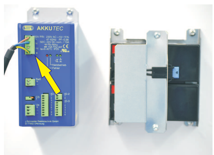
Connect the AKKUTEK to the mains (230 V AC)
